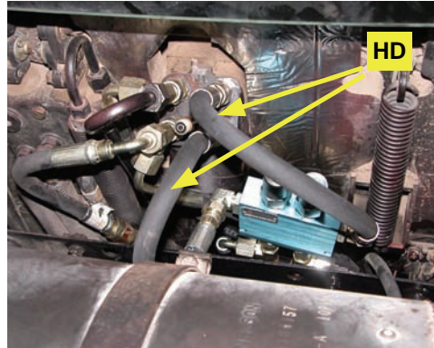
Figure 4b: CBV hoses installed at orbital
