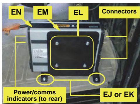
Figure 1b: ECU installed
